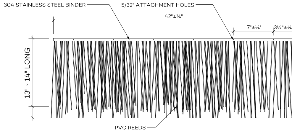
FIELD SHINGLE DETAIL
